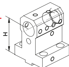
W1417 D32 - H=55 mm (Ø32 mm) Z2417 D32 - H=70 mm (Ø32 mm) Z7417 D32 - H=80 mm (Ø32 mm)
