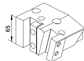
R1452 - 20x20 mm
